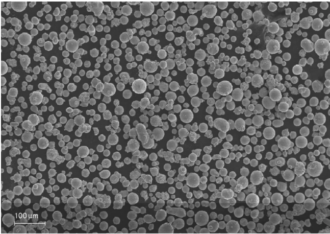
SEM micrograph of EOS StainlessSteel CX powder
