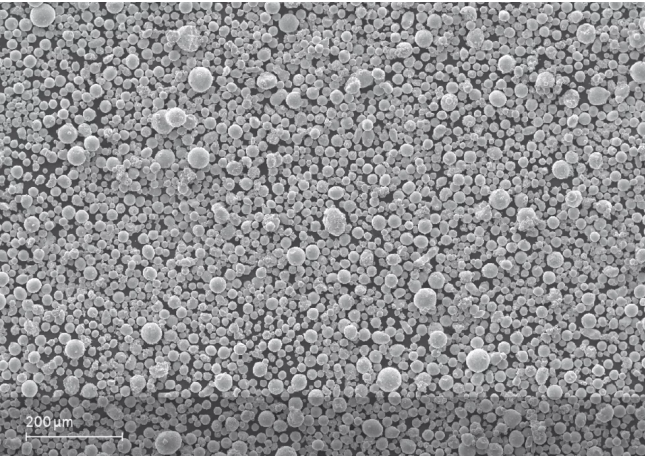
SEM micrograph of EOS StainlessSteel SuperDuplex powder
