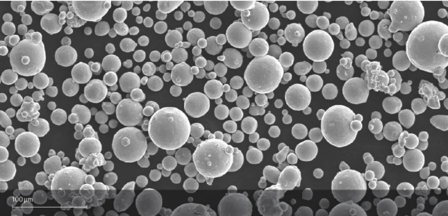
SEM micrograph of EOS Titanium Ti64 Grade 23 powder
